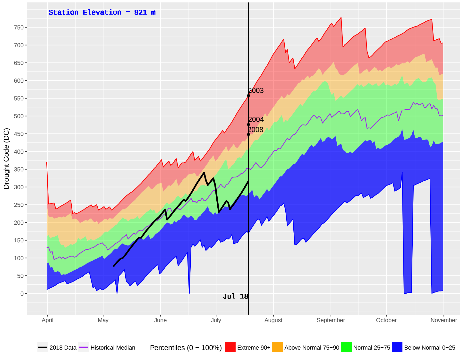
KNIFE (225) : Historical (1991–2016) and Current (2018) Daily Drought Code (DC)
