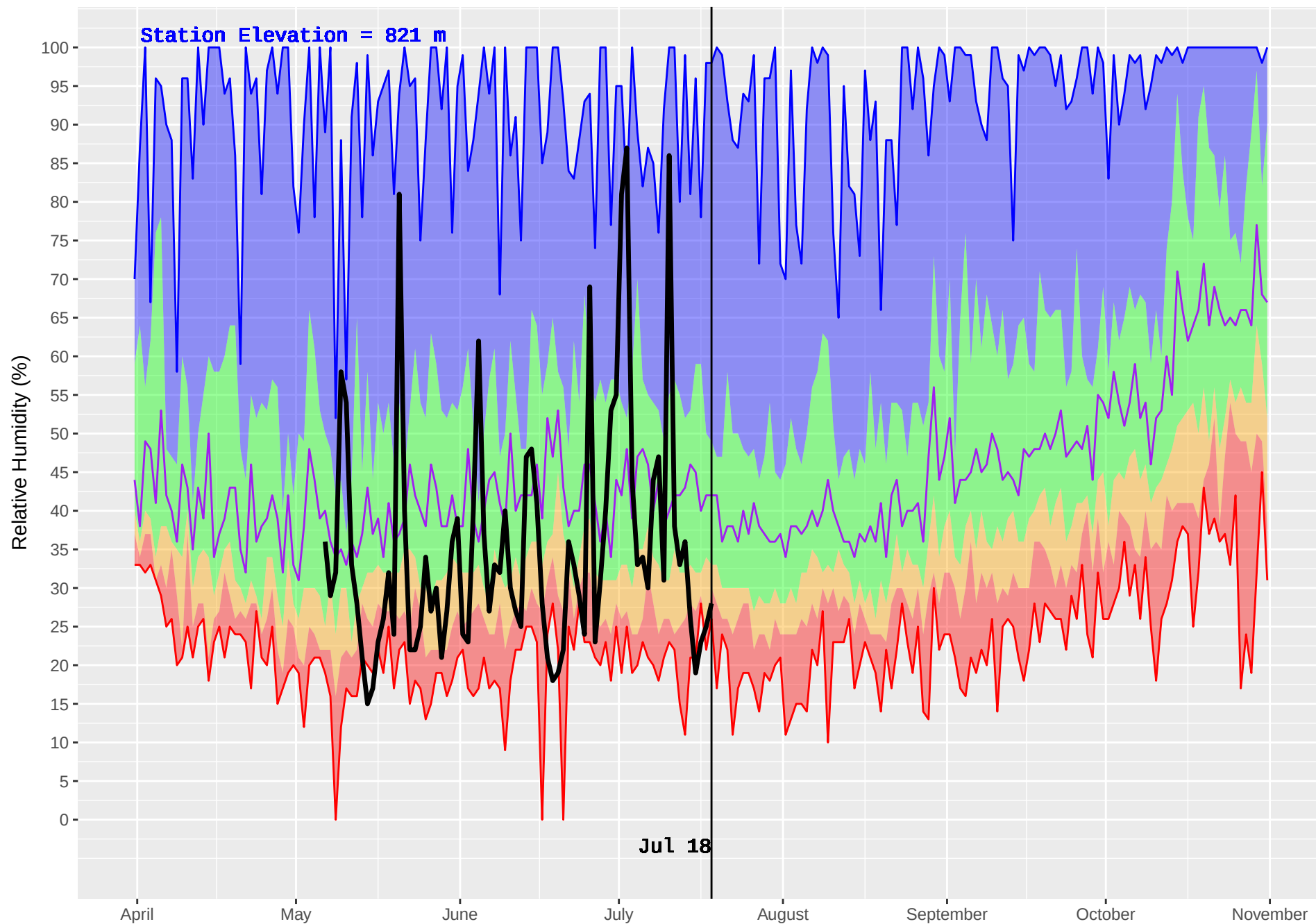
KNIFE (225) : Historical (1991–2016) and Current (2018) Daily Relative Humidity
