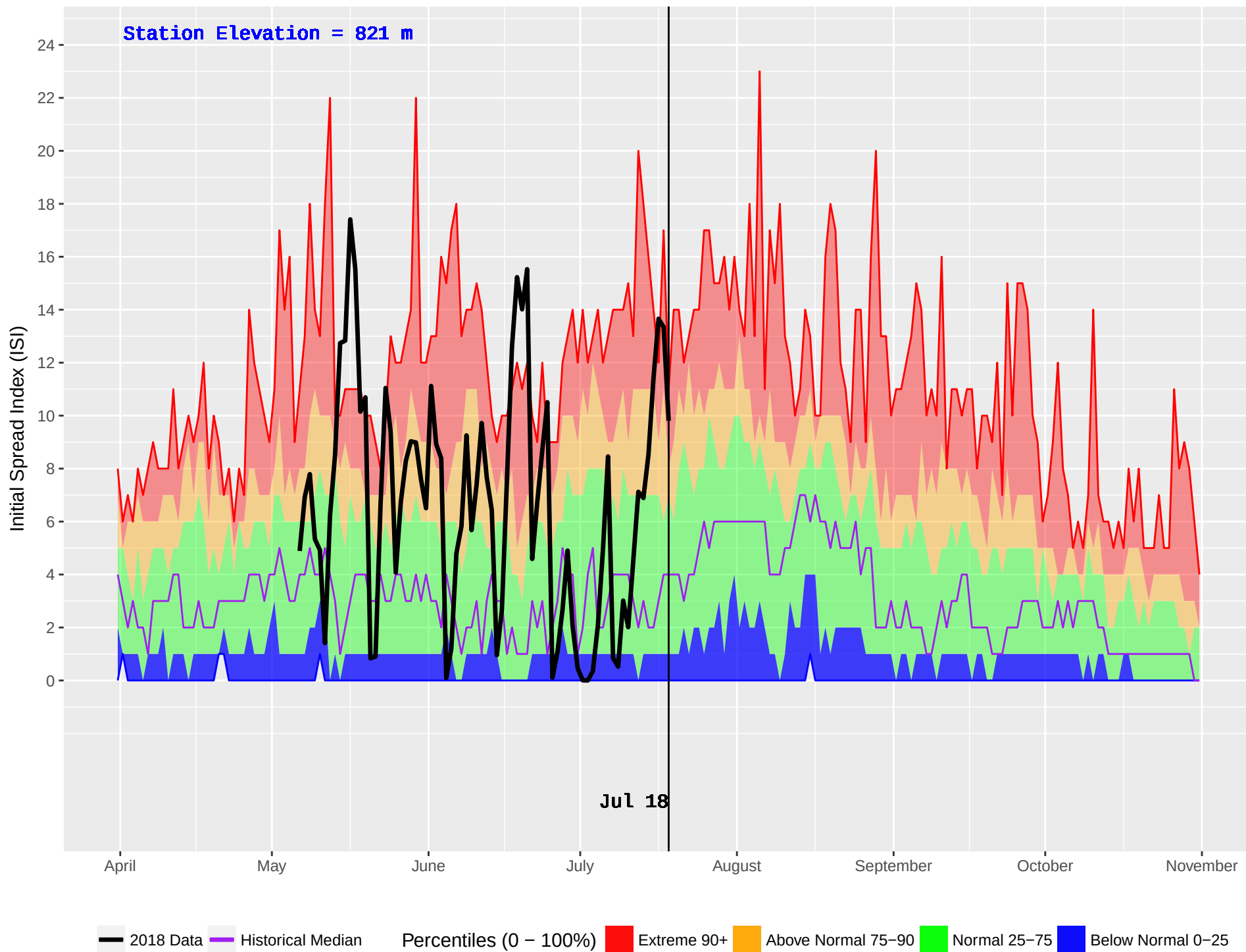
KNIFE (225) : Historical (1991–2016) and Current (2018) Daily Initial Spread Index (ISI)
