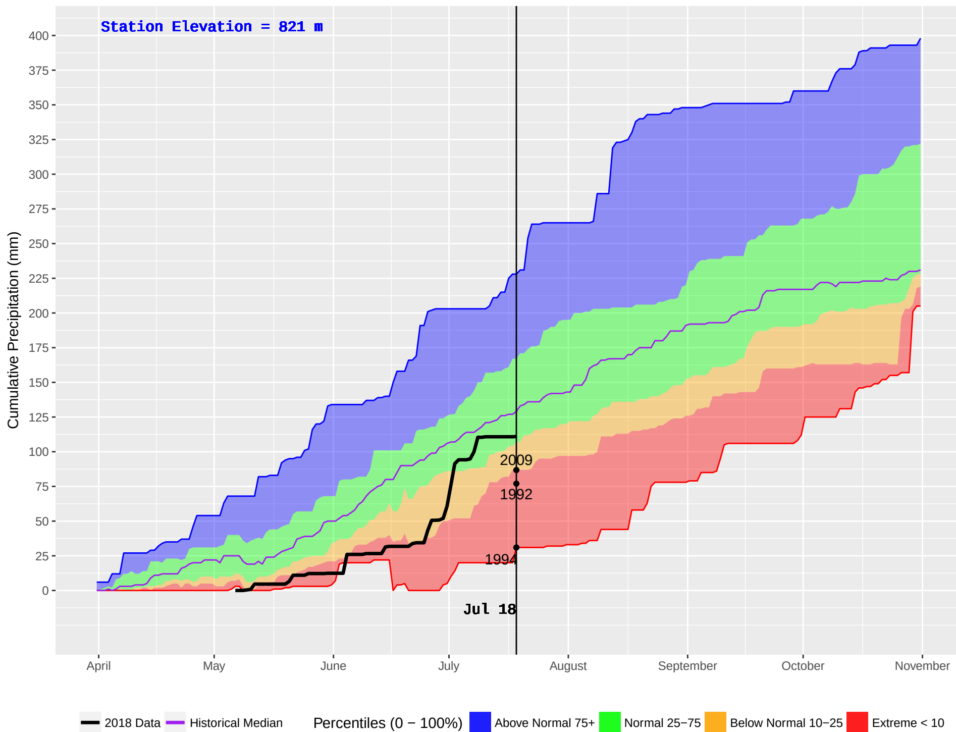
KNIFE (225) : Historical (1991–2016) and Current (2018) Daily Cumulative Precipitation
