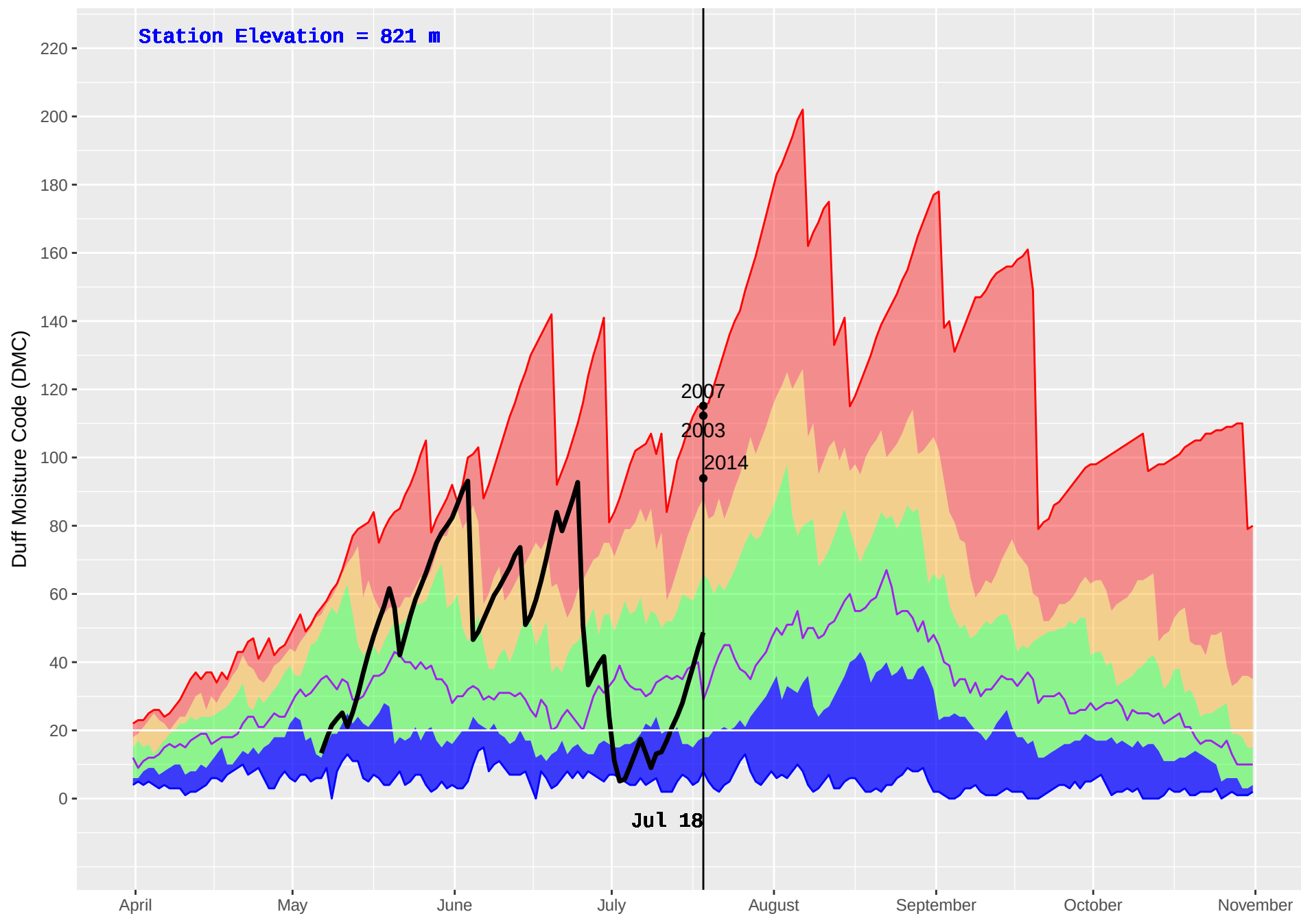
KNIFE (225) : Historical (1991–2016) and Current (2018) Daily Duff Moisture Code (DMC)
